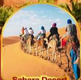
Sahara Desert
